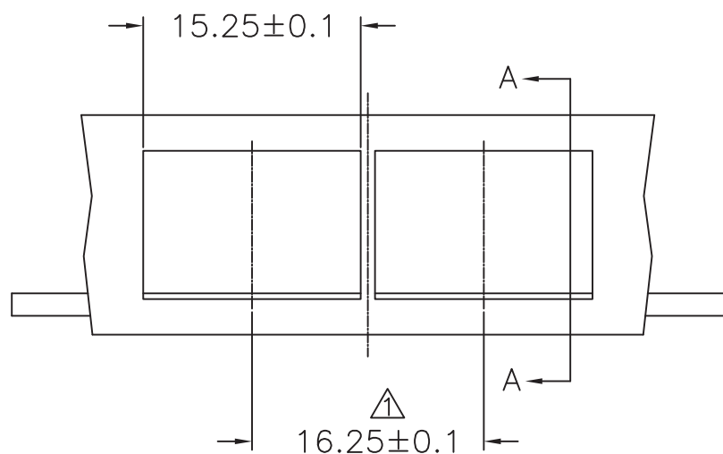
RECOMMENDED BEZEL DESIGN
